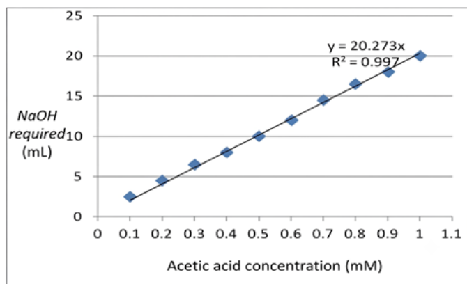
Figure 1: Standard graph for lipase enzyme activity
