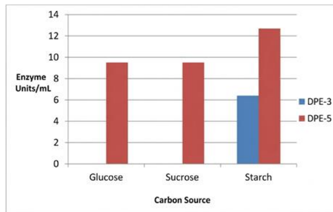
Figure 5: Effect of carbon sources on lipase enzyme production.
