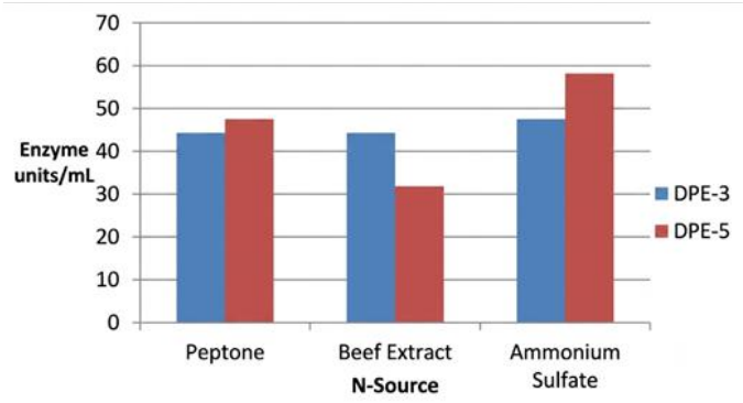
Figure 6: Effect of nitrogen sources on lipase enzyme production.
